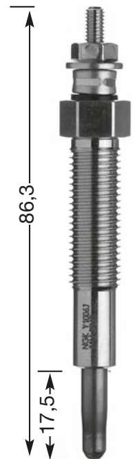
Y1006 J M 10 x 1.25 12 Hex 11 V
