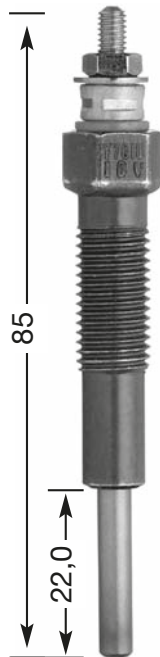
Y-701 U M 10 x 1.25 12 Hex 10 V
