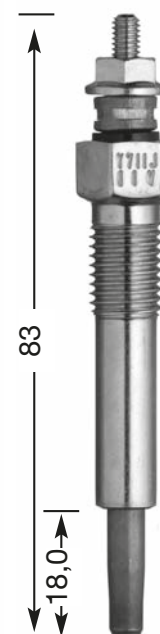
Y-711 J M 10 x 1.25 12 Hex 11 V
