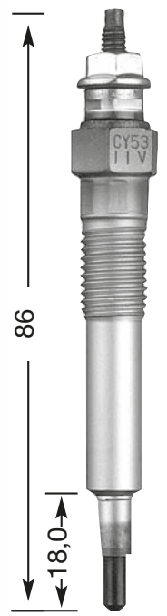
CY 03 M 10 x 1.25 12 Hex 11 V
