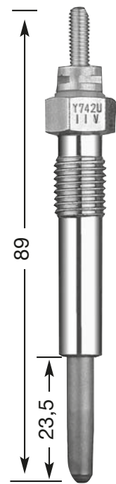
Y-742 U M 10 x 1.25 12 Hex 11 V
