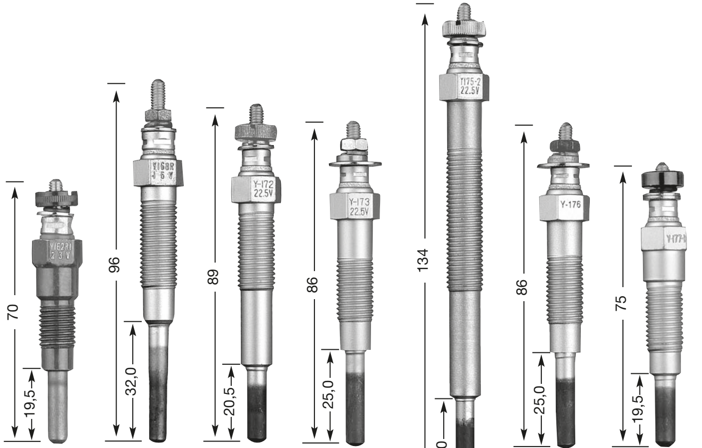
Y-162 R1 M 10 x 1.25 12 Hex 23 V
