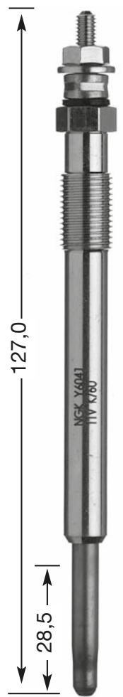
Y-604 J M 10 x 1.0 10 Hex 11 V
