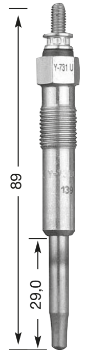
Y-731 U M 10 x 1.0 10 Hex 11 V DP 9
