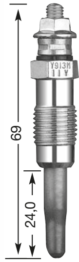
Y-913 M M 12 x 1.25 12 Hex 11 V
