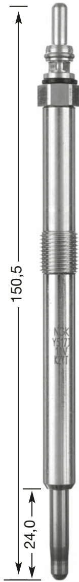
Y-517 J M 10 x 1.0 10 Hex 11 V DP 66
