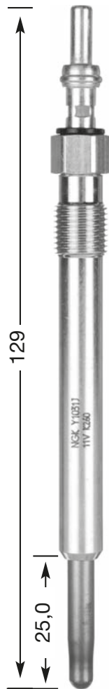
Y1031 J M 10 x 1.0 10 Hex 11 V DP 71
