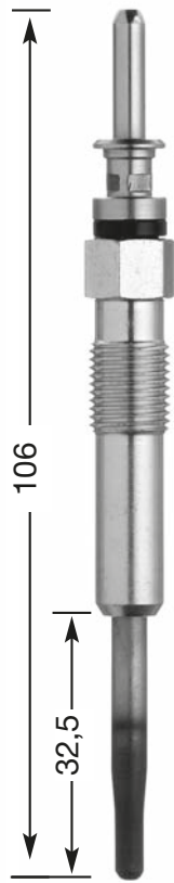
Y-547 AS M 10 x 1.0 10 Hex 5 V DP 47
