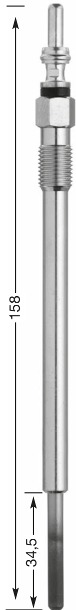
Y-9003 AS M 9 x 1.0 9 Hex 4,4 V DP 78
