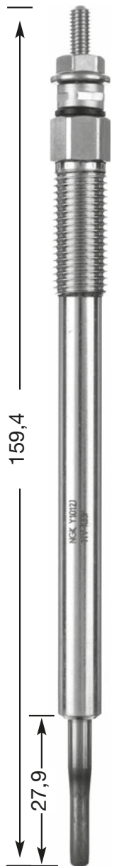
Y1012 J M 10 x 1.25 10 Hex 11 V DP 65
