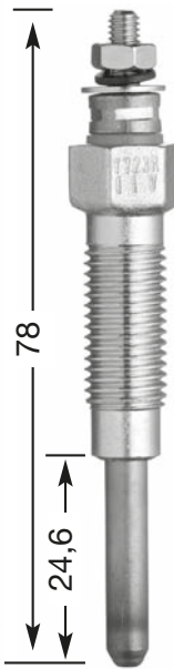
Y-723 R M 10 x 1.25 12 Hex 11 V
