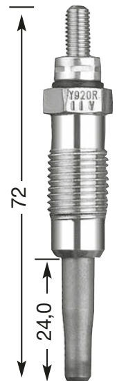
Y-920 R M 12 x 1.25 12 Hex 11 V
