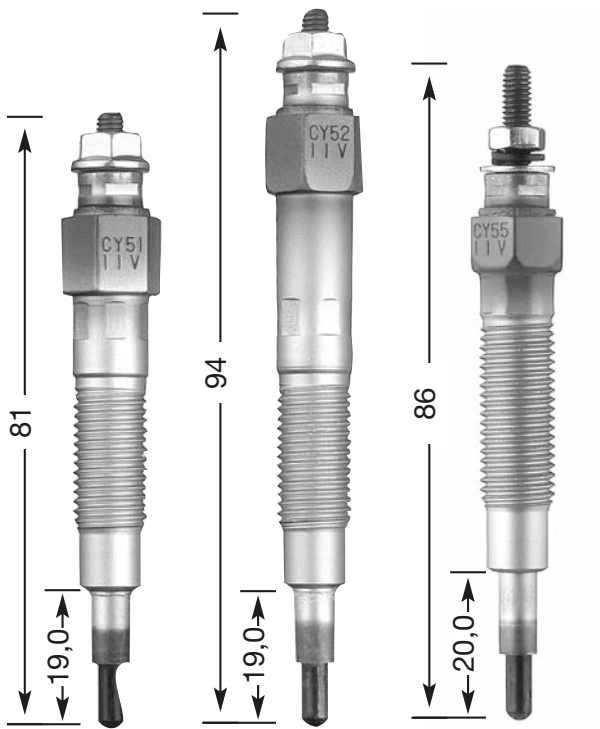
CY 51 M 10 x 1.25 12 Hex 11 V
