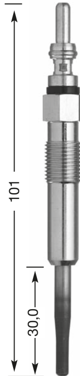
Y-607 AS M 10 x 1.0 10 Hex 5 V DP 50
