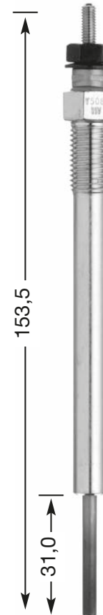
Y-508 J M 10 x 1.25 12 Hex 11 V
