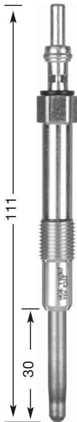
Y1030 J M 10 x 1.0 10 Hex 11 V DP 70
