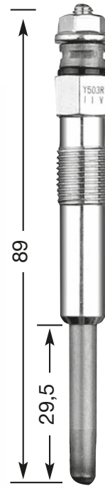
Y-503 R M 10 x 1.0 10 Hex 11 V
