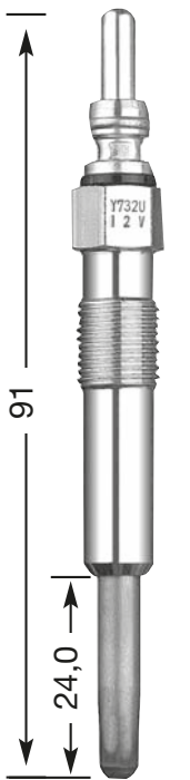
Y-732 U M 10 x 1.0 10 Hex 12 V DP 4
