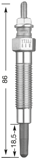
Y-733 J M 10 x 1.25 12 Hex 11 V DP 13
