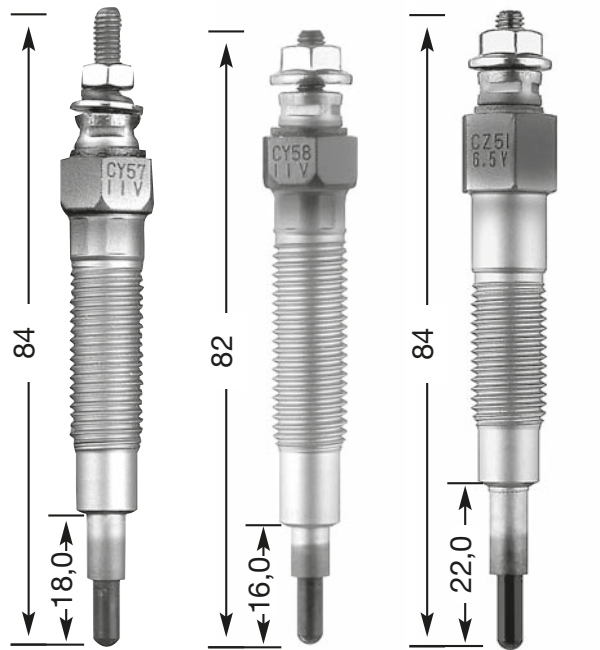
CY 57 M 10 x 1.25 12 Hex 11 V
