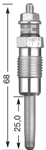
Y-927 R M 12 x 1.25 12 Hex 11 V
