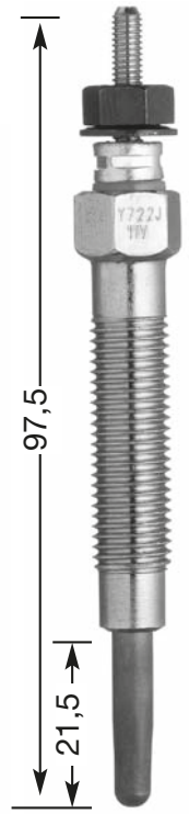
Y-722 J M 10 x 1.25 12 Hex 11 V
