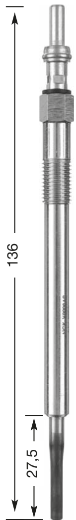
Y8008 AS M 8 x 1.0 8 Hex 11 V DP 74
