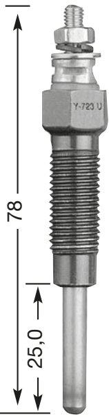
Y-723 U M 10 x 1.25 12 Hex 8 V
