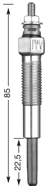
Y-701 J M 10 x 1.25 12 Hex 11 V DP 39
