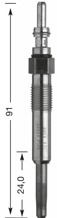
Y-732 J M 10 x 1.0 10 Hex 12 V DP 4
